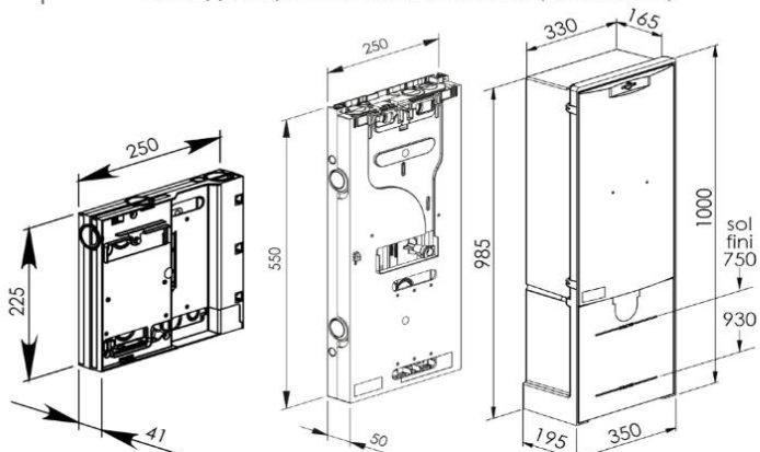
Coffret CIBE®
