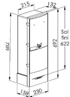
Borne CIBE®
